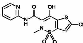
Figure 1. Structure of Lornoxicam
