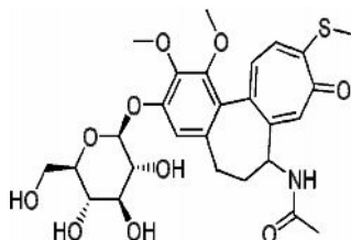
Figure 2. Structure of Thiocolchicoside
