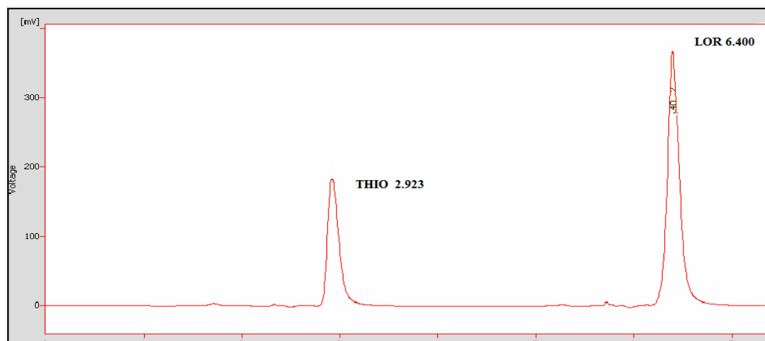
Figure 3 HPLC Chromatogram of LOR (40 \mu g/ml) and THIO(20 \mu g/ml)
