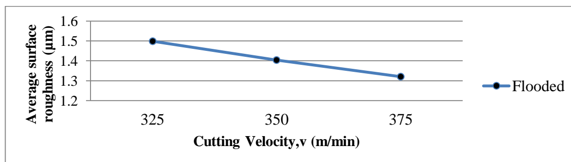
Figure 1: Effect of cutting velocity on surface roughness
