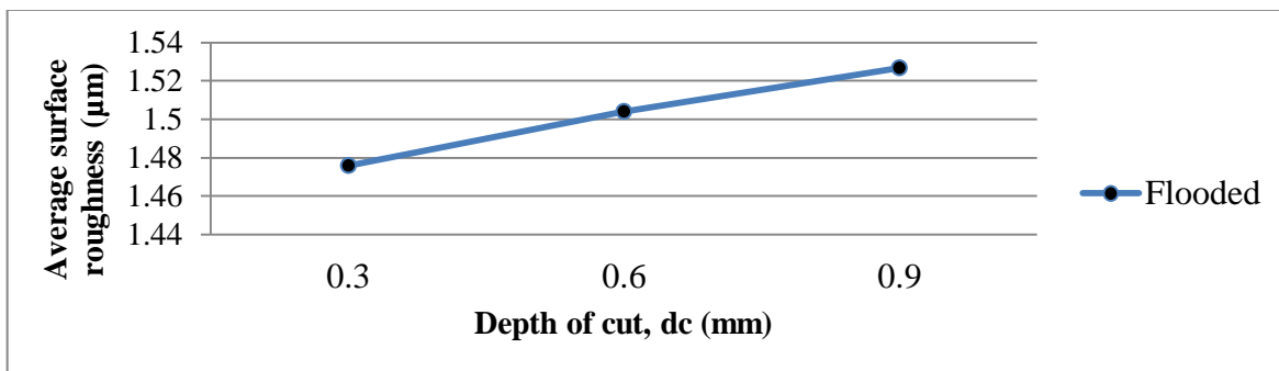
Figure 3: Effect of depth of cut on surface roughness
