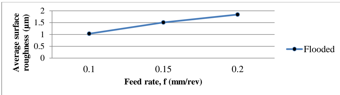
Figure 2: Effect of cutting feed on surface roughness
