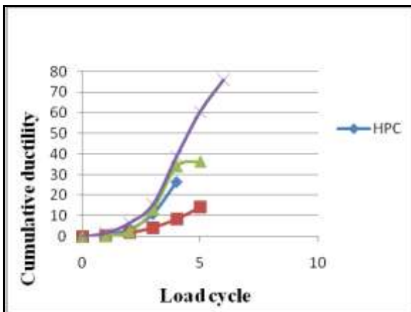
Fig.18.Comparison of Cumulative Ductility factor
