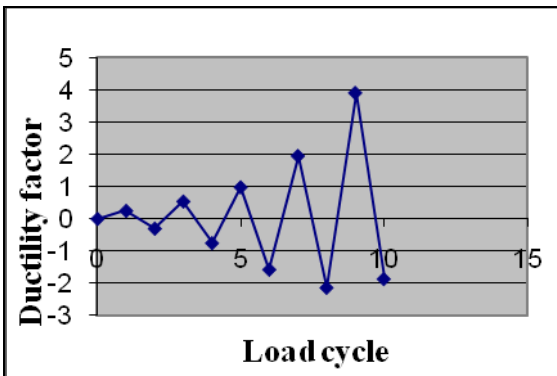
Fig.10.Behaviour of Crimped fiber RC beam
