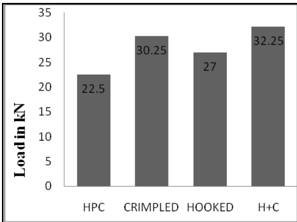
Fig.18.Comparison of Ultimate Load
