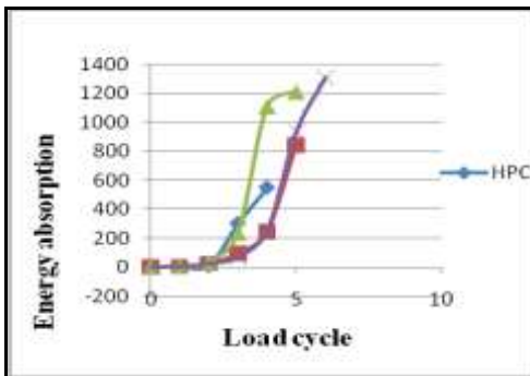
Fig.19.Comparison of Energy Absorption
