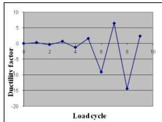
Fig.8.Variation of Ductility Factor with Load Cycle
