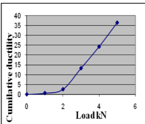
Fig.7.Loop Diagram for HPC Beam Behaviour of Hooked end Fiber RC beam
