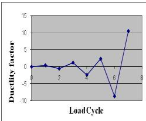
Fig.3.Behaviour of conventional concrete beam
