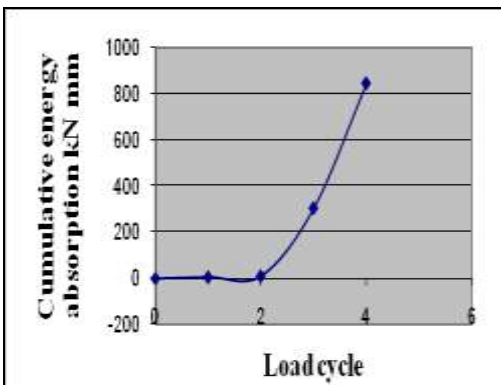
Fig.5.Variation of cumulative ductility factor with load cycle
