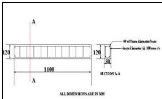
Fig.1. Reinforcement Details
