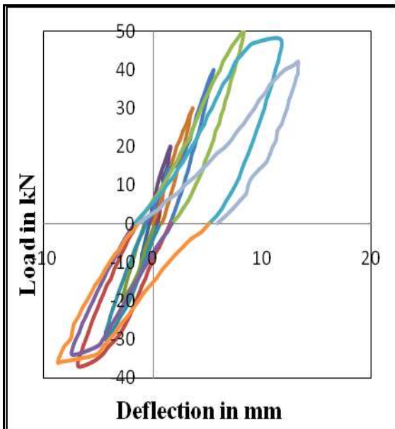
Fig.16. Loop Diagram for Hybrid Beam
