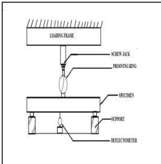
Fig.2.Experimental Setup
