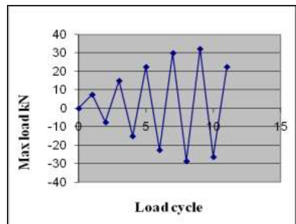
Fig.15.Load Sequence Diagram
