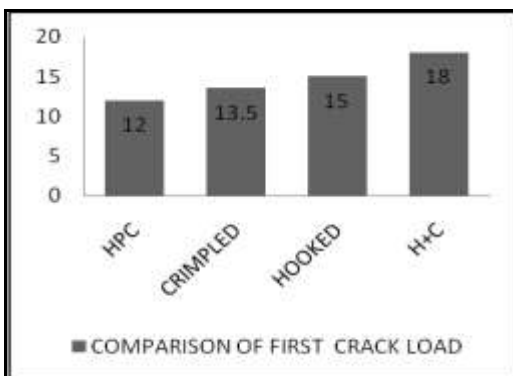
Fig.17. Comparison of First Crack Load
