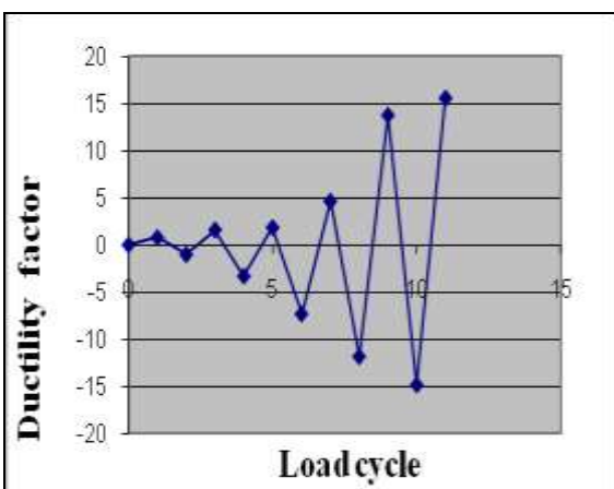
Fig.14.Variation of Ductility Factor with Load Cycle
