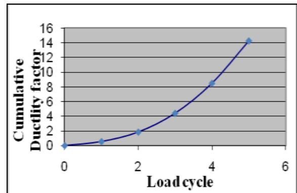
Fig.11.Variation of Ductility Factor with Load Cycle
