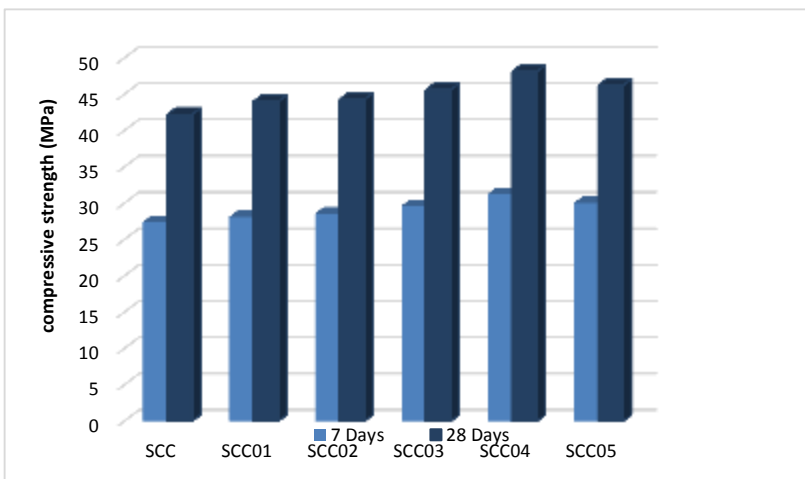
Figure 2.Compressive strength of Self Compacting Concrete
