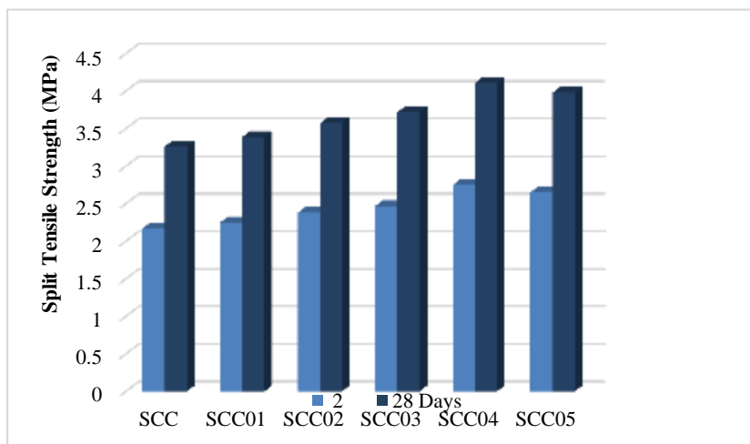
Figure 3.Split tensile strength of Self Compacting Concrete
