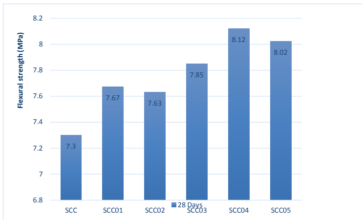
Figure 4. Flexural strength of Self Compacting Concrete
