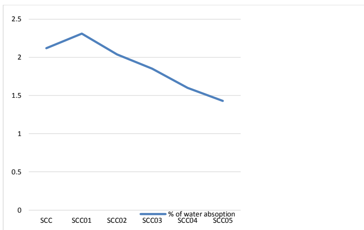
Figure 5. Water absorption of Self Compacting Concrete
