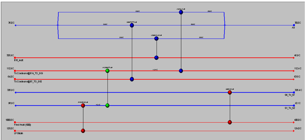
Figure 4. Retrofit HEN
