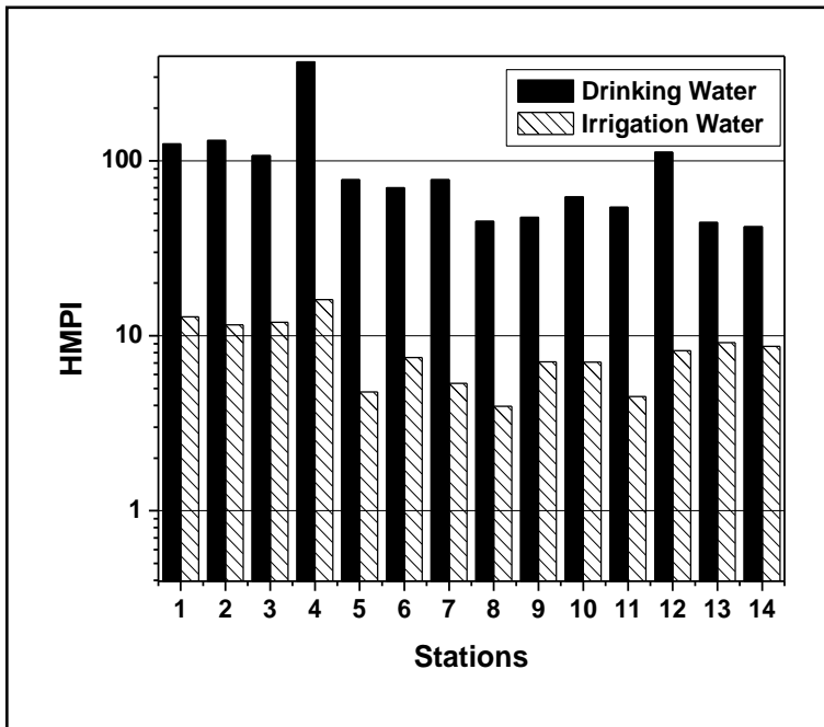
Fig. (4): HMPI of Drinking and Irrigation water of Damietta Nile Branch in Damietta Governorate
