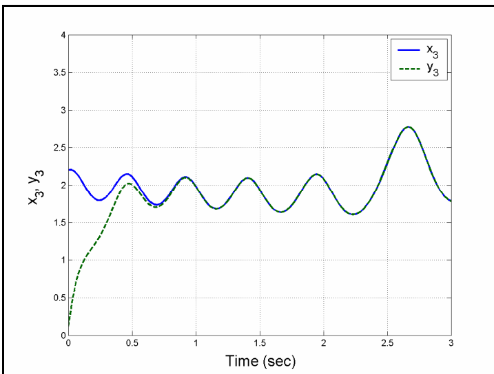
Figure 8. Complete synchronization of the states x_3 and y_3
