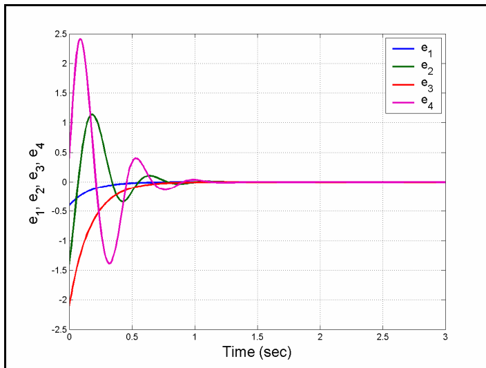
Figure 10. Time-history of the synchronization errors e_1, e_2, e_3, e_4
