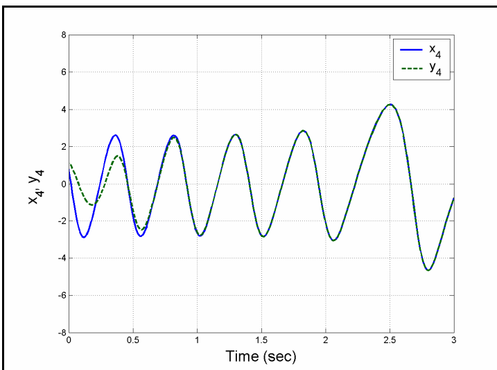
Figure 9. Complete synchronization of the states x_4 and y_4
