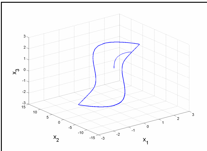
Figure 1. 3-D Projection of the Conservative Chaotic System on the (x_1, x_2, x_3) space
