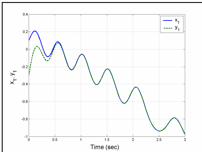
Figure 6. Complete synchronization of the states x_1 and y_1
