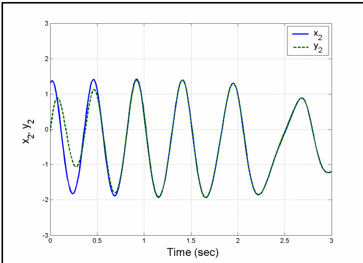
Figure 7. Complete synchronization of the states x_2 and y_2
