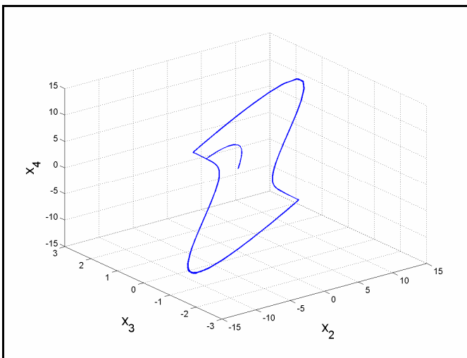
Figure 4. 3-D Projection of the Conservative Chaotic System on the (x_2, x_3, x_4) space
