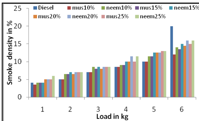
Figure-6. Bp Vs Smoke density
