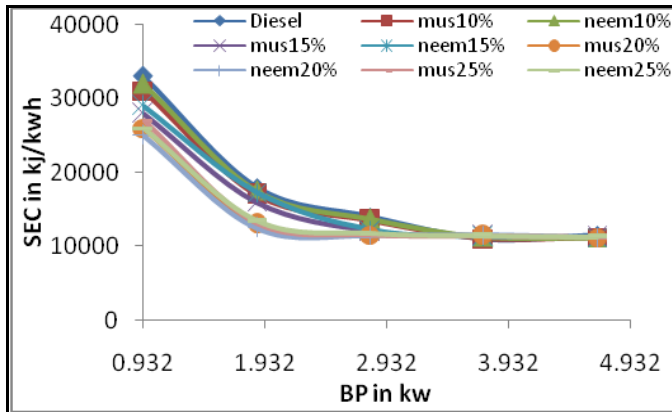
Figure-3. Bp Vs SEC
