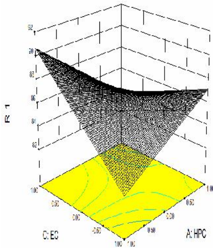
Figure 6: R 1 (Response surface plot) of EC – HPC
