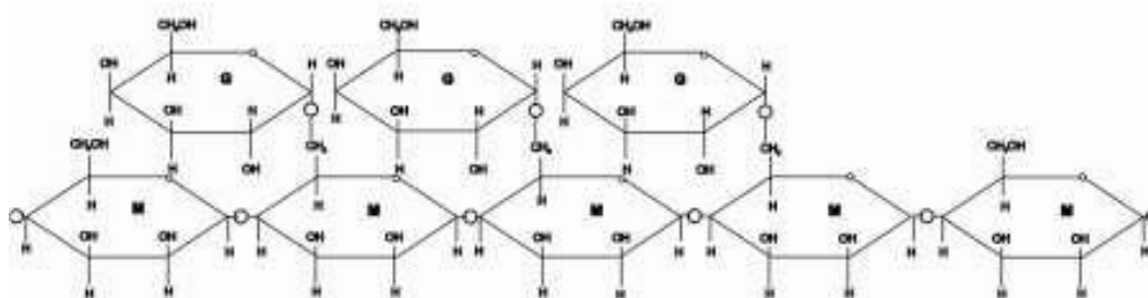
Fig.3: Structure of octasaccharide showing 1-4 and 1-6 linkages
