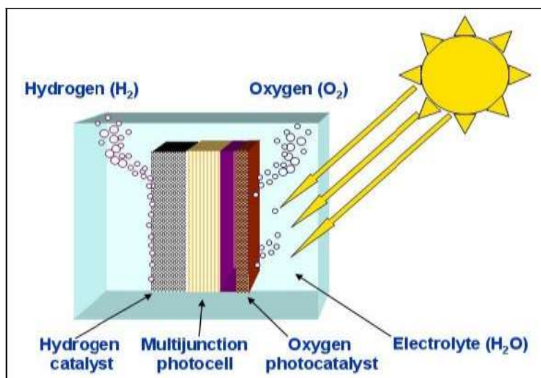
Figure 4: Basic structure of a Photoelectrode
