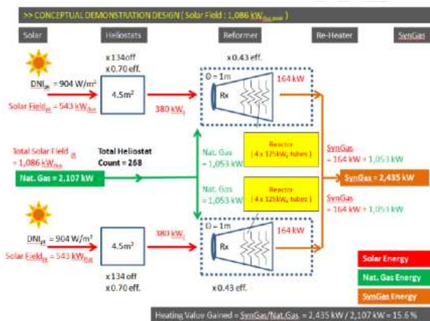
Figure 6 : Proposed solar Gas Power Plant
