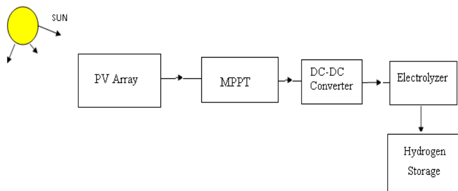
Figure 2 : Schematic of PV – hydrogen production system
