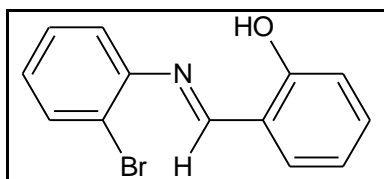
Figure 1. Primary ligand 2-{(E)-[(2-bromophenyl)imino]methyl}phenol
