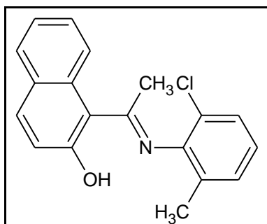
Figure 2. Secondary ligand 1-[(1E)-N-(2-chloro-6-methylphenyl)ethanimidoyl]naphthalen-2-ol
