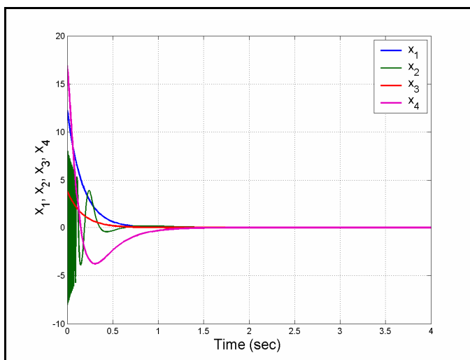
Figure 6. Time-history of the controlled states x_1, x_2, x_3, x_4
