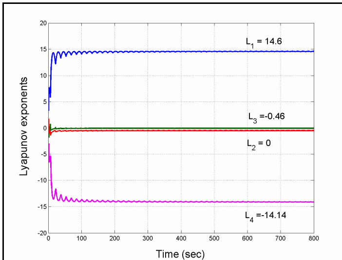
Figure 5. Lyapunov exponents of the Novel 4-D Coupled Van der Pol Conservative Chaotic System
