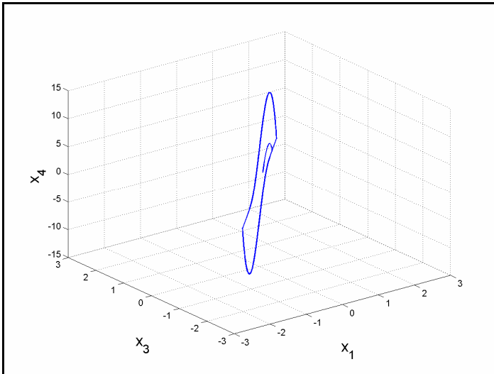
Figure 3. 3-D Projection of the Conservative Chaotic System on the (x_1, x_3, x_4) space
