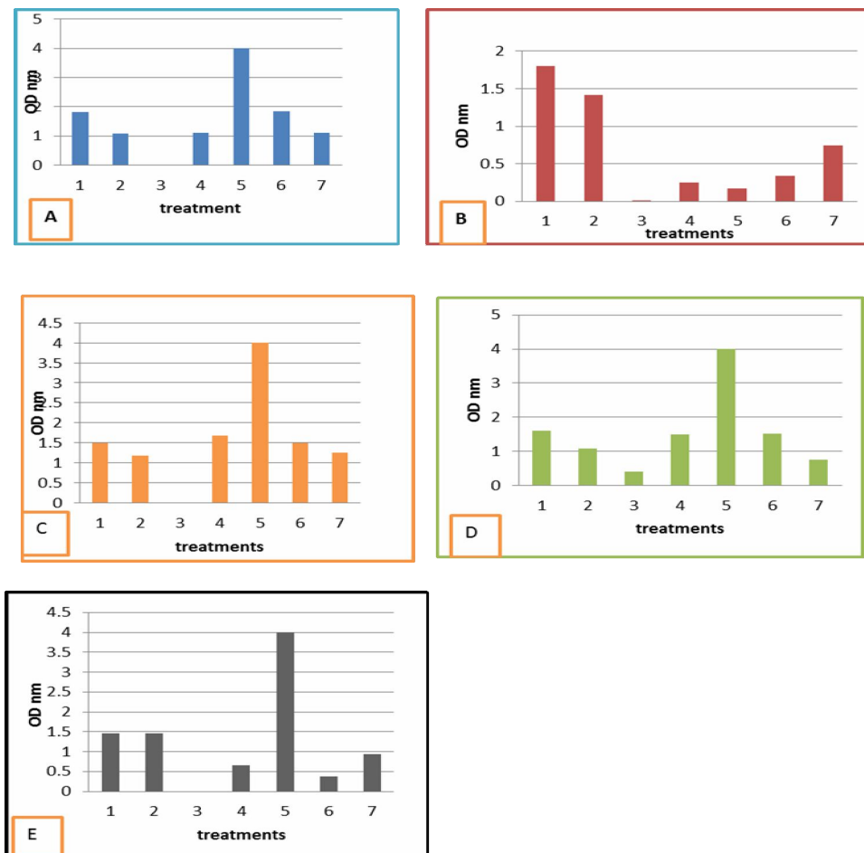
Figure (2) antibacterial activity of plants extract against different pathogenic bacteria A, E.coli ; B, S. aureus ; C, Klebsilla pnemoniae ; D,, Serratia Spp ; E; Aeromonas hydrophillia was . 1,positive control; 2, glycyrrihza glabra;3, Hordeum vulgare ;4, Origanum vulgare ; 5, Salvia officinalis ; 6, Punica granatum ; 7, Zingiber officinale .
