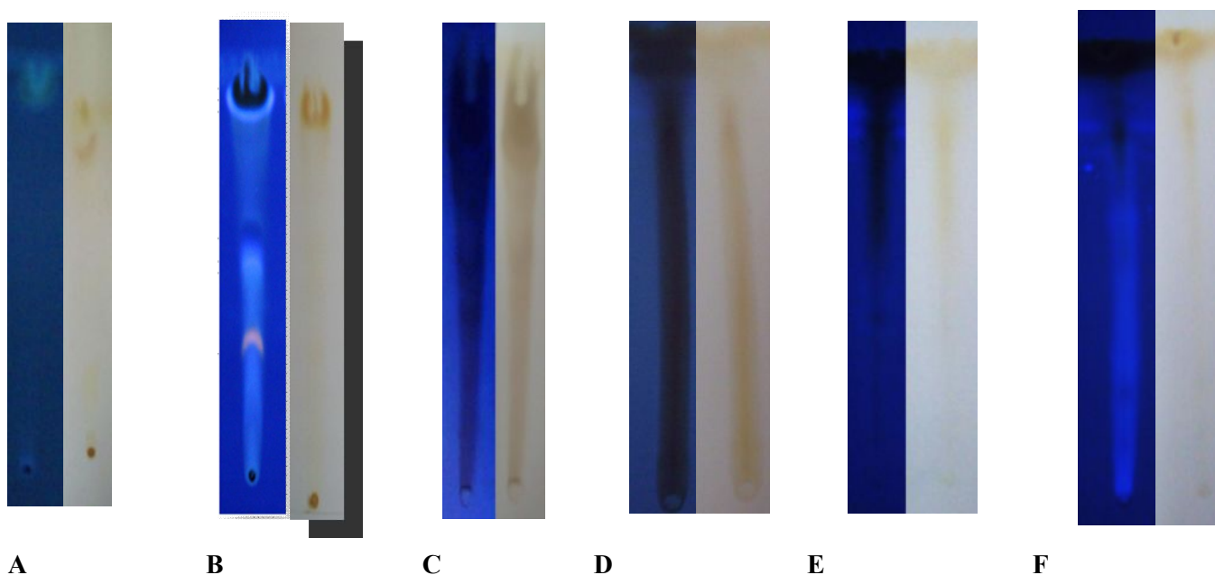
Figure (1) thin layer chromatography profile of plant extract using as antibacterial activity under visible and UV light (312 nm) A, barley ; B, Liquors; C, Origanum vulgare ; D, Pomegranate cortex; E, Ginger; F, sage .
