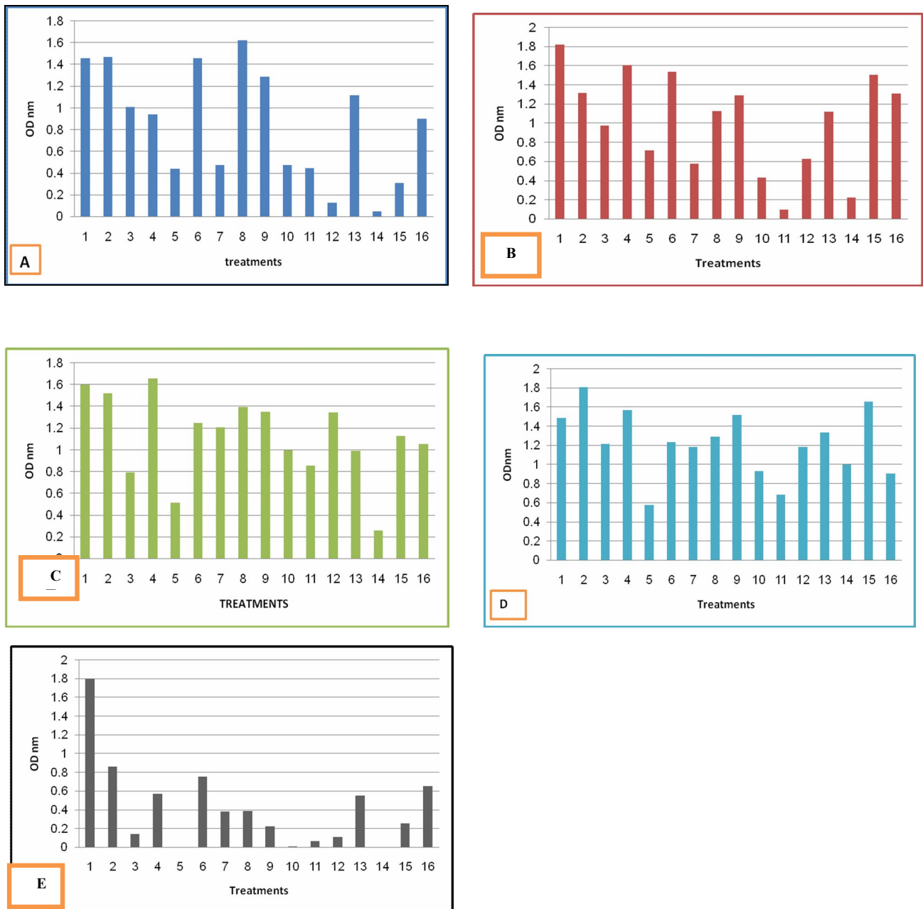
Figure (3) antibacterial activity of plants extract against different pathogenic bacteria A, E.coli; B ,S.aureus; C, Klebsilla pnemoniae ; D, , Serratia Spp; E; Aeromonas
