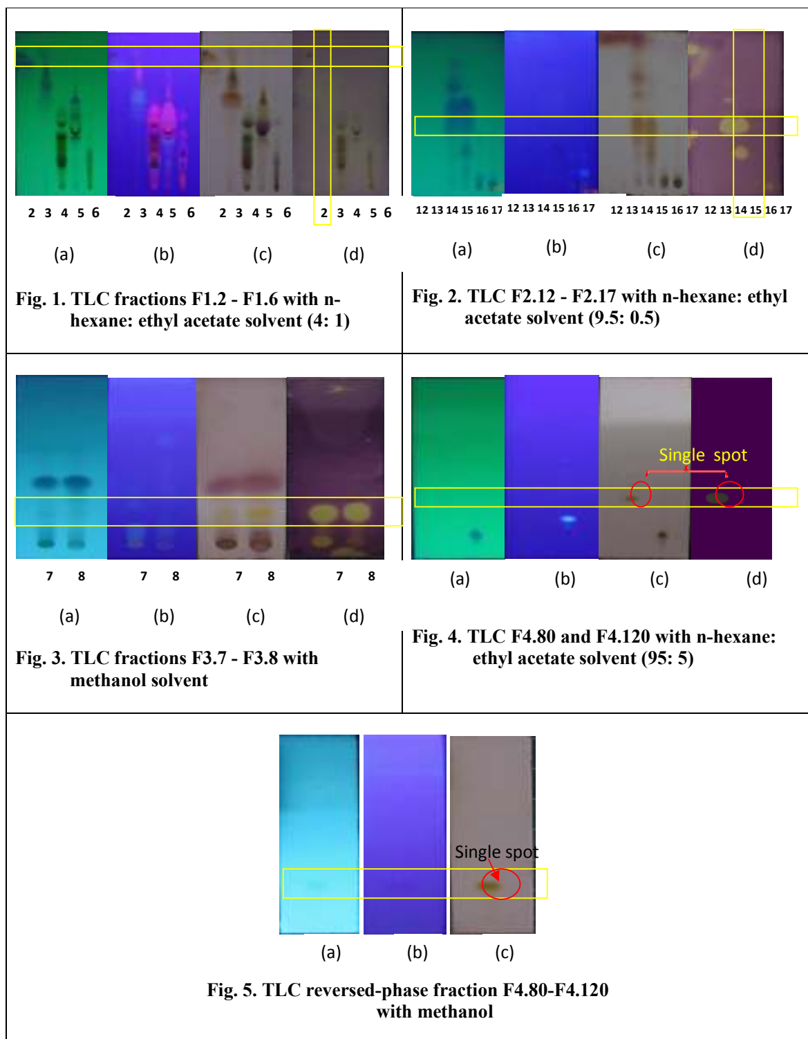
Fig. 1-5. Isolation and identification of active antioxidant compounds fraction of ethyl acetate (a) Viewed under UV 254 nm, (b) Viewed under UV 365 nm, (c) Sprayed with 10% H 2 SO 4 in ethanol, and (d) Dipped in a solution of 0.05% DPPH in methanol
