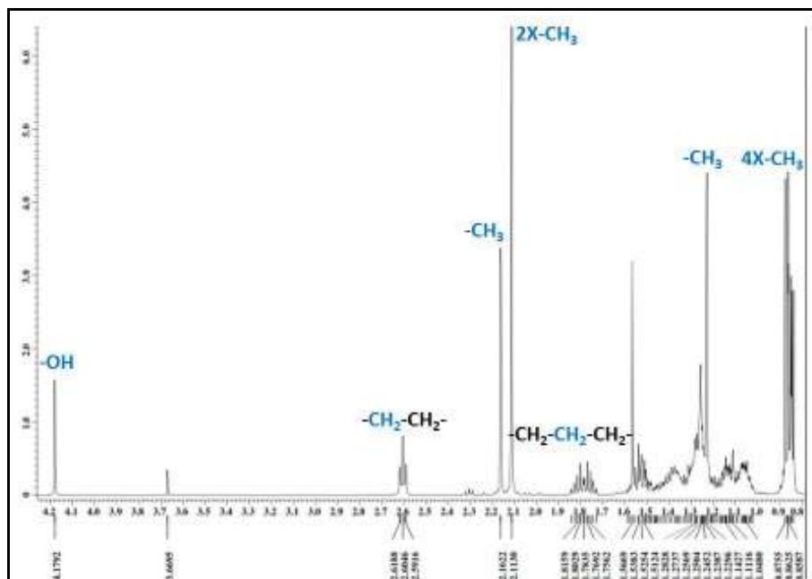
Fig. 7. ^1\text{H-NMR} spectrum of target compounds (500 MHz in chloroform-D)
