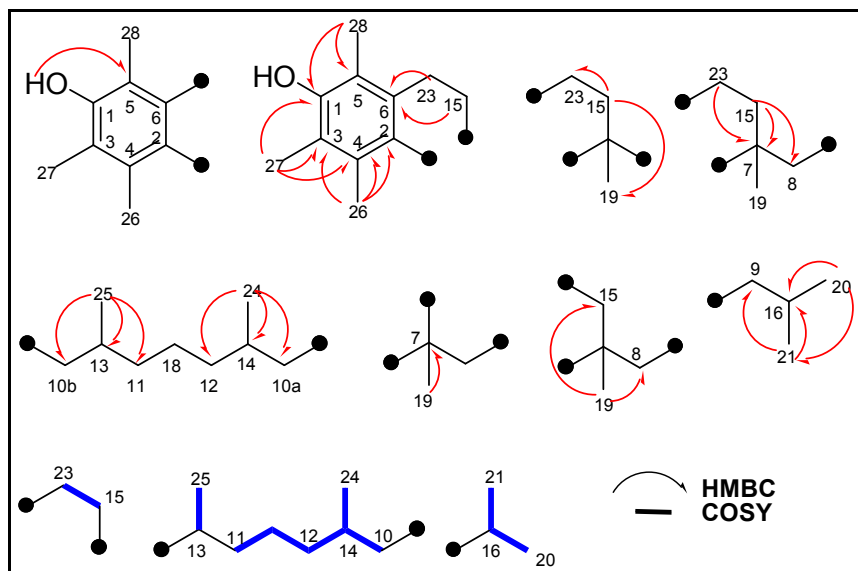
Fig. 9. Fragments of the target compound
