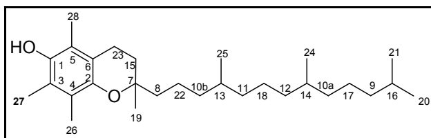
Fig.10. Alleged target compound structure
