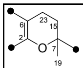
Fig 8. Alleged cyclic / furan ring formed by C2, C6, C7, C15 and C23
