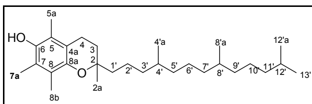
Fig.11. Structure of \alpha -tocopherol
