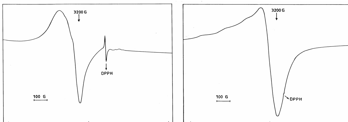
Figure 1. The X-band EPR spectrum of the copper complex in DMSO at 300 K (a) and 77 K (b)
