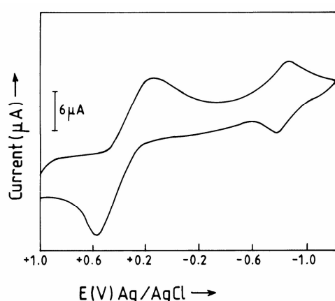
Figure 2. Cyclic voltammogram of copper complex in MeCN
